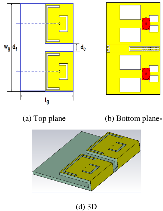
Figure 2. Structure of Proposed triple-band MIMO antenna.
