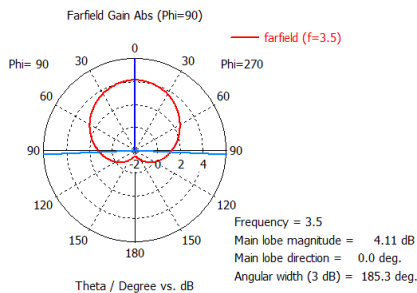
(b) At 3.5 GHz
