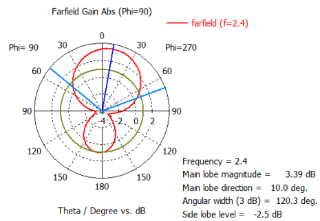
(a) At 2.4 GHz
