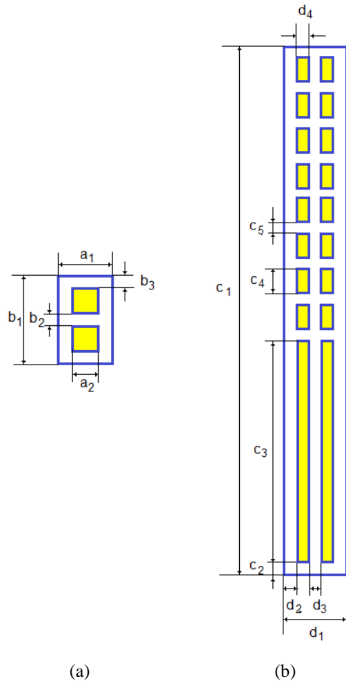
Figure 3. The slot loaded structure (a) double square shape (b) periodic rectangular shape.
