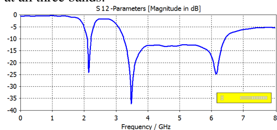
Figure 9. The S12 parameters of decoupling structure using “slot and variation” DGS.
