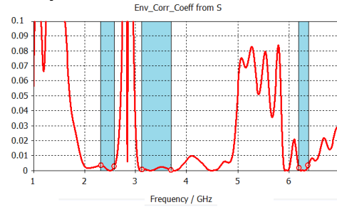
Figure 11. Correlation Factor |\rho_{12}| curve for the proposed MIMO antenna.
