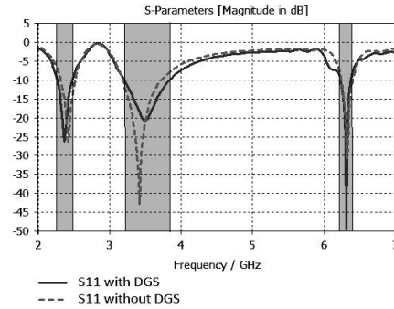
Figure 4. The reflection coefficient of antenna with and without double rectangular DGS structures.
