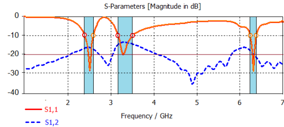
Figure 6. The S parameters of MIMO antenna with distance from feed to feed is 0.5\lambda at 6.3 GHz.
