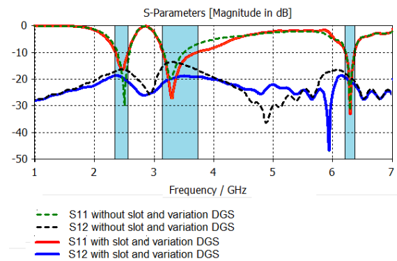
Figure 10. The S parameters of MIMO antenna with and without slot and variation DGS structures at the distance of 4 mm from edge to edge.
