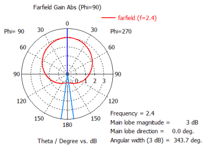
(a) At 2.4 GHz
