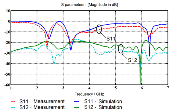
Figure 15. Measured and simulated results of S parameter of the proposed MIMO PIFA antenna.
