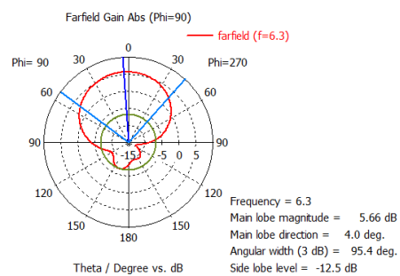
(c) At 6.3 GHz
