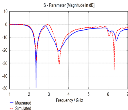
Figure 13. Measured and simulated results of S11 parameter of the proposed single PIFA antenna.
