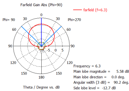
(c) At 6.3 GHz
