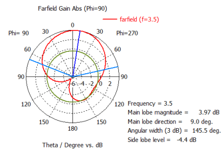
(b) At 3.5 GHz
