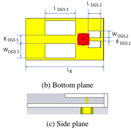
Figure 1. Structure of the proposed triple-band PIFA antenna.
