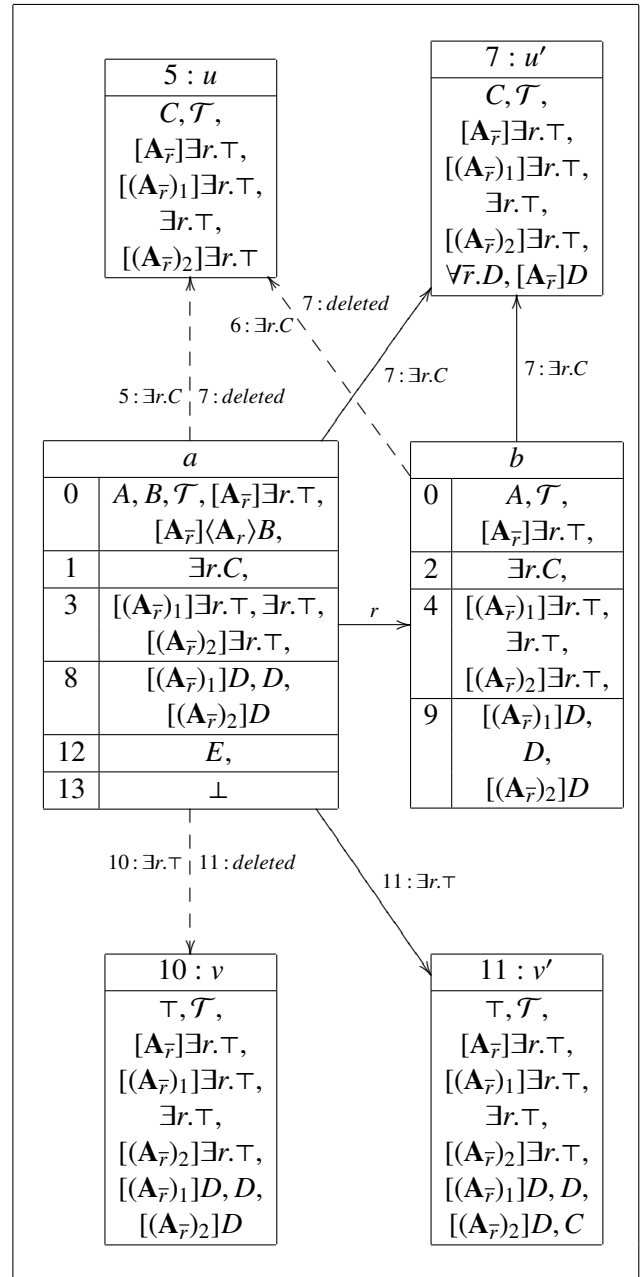
Fig. 1. An illustration for Example 3.
