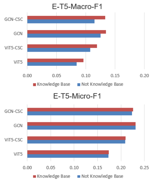
Figure 8. Results of knowledge base by single models.
